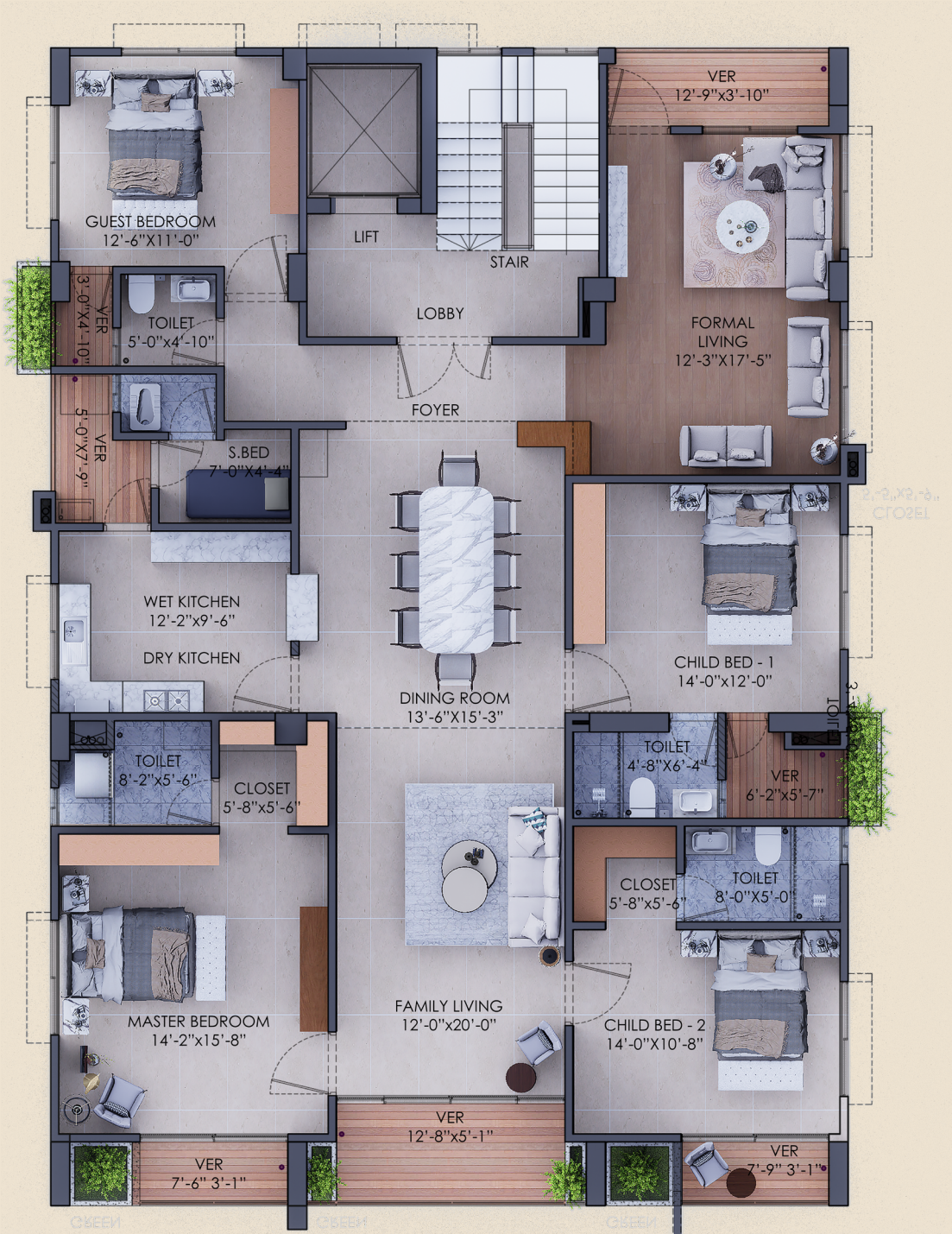
1 TYPICAL FLOOR PLAN
