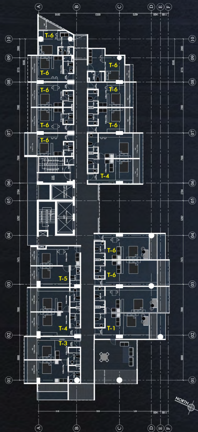
Typical Floor Plan (10th Floor & 6th Floor)
